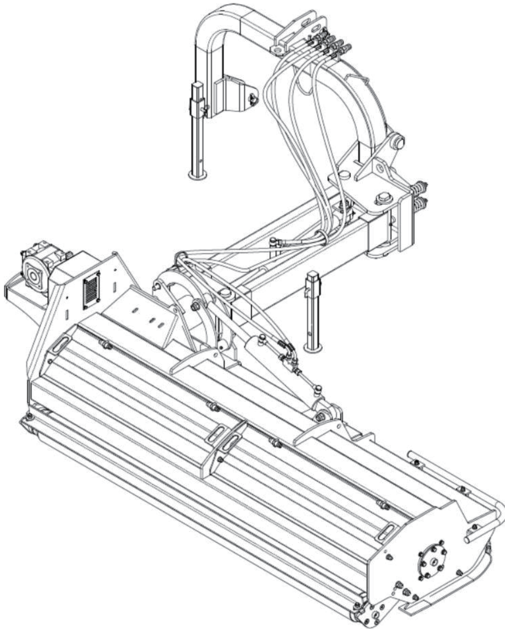
Figure 1-8: Installing Rake Sub-Assembly and Oil Pipes Fixation
